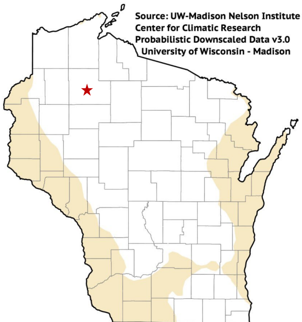
Change in JJA PRCP (%), SSP245: 2041-2060 minus 1981-2010
