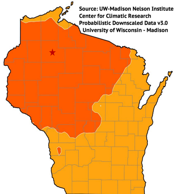
Change in SON TMEAN, SSP245: 2041-2060 minus 1981-2010
